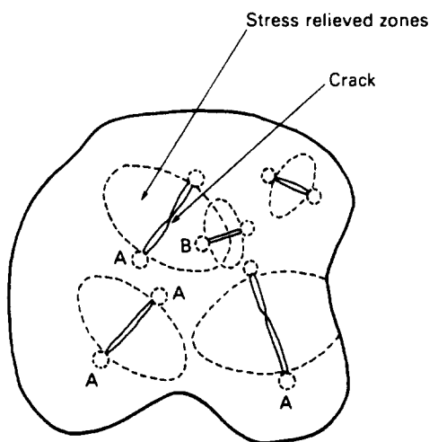
Fig. 2. Schematic of stress relieved zone and crack propagation sites (after Van Mier[12]): A, potential crack extension site; B, unlikely site for crack growth.
