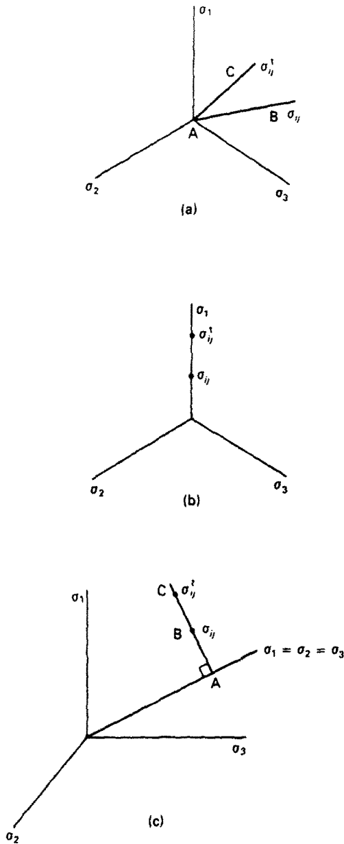
Fig. 5. Relative position of \sigma_{ij}^d and \sigma_{ij} : (a) in the deviatoric plane ( \sigma_{kk}^d = \sigma_{kk}^0 ) (b) in the deviatoric plane \sigma_1 = \sigma_3 ; (c) in principal stress space.
